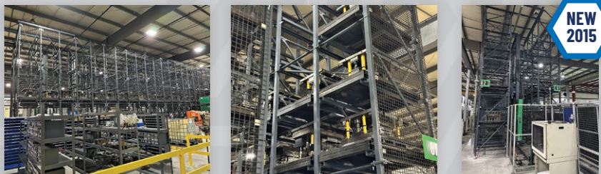
Toyota 270-Station Die Storage Rack System w. Auto Retriever
