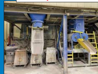
Complete Concrete Batch Plant
