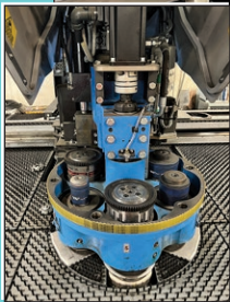
33 Ton Euromac Model MBX 6 Plus 1250/30-2250 CNC Turret Punch
