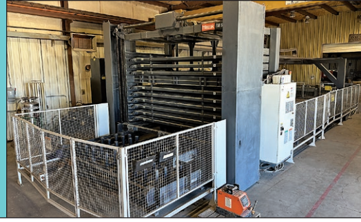
2,500 Watt 5' x 10' Mazak Super Turbo-X510MK II CNC CO2 Laser w/ 10-Shelf FMS
