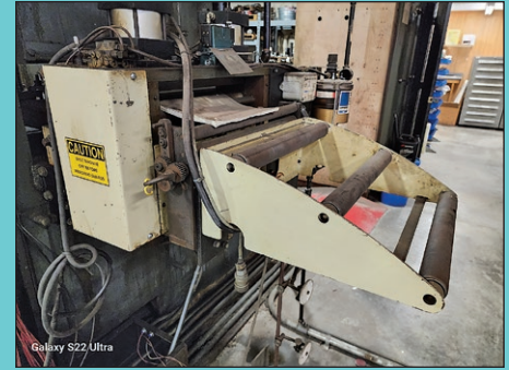
CW Model SMX-18 Servo Feeder
